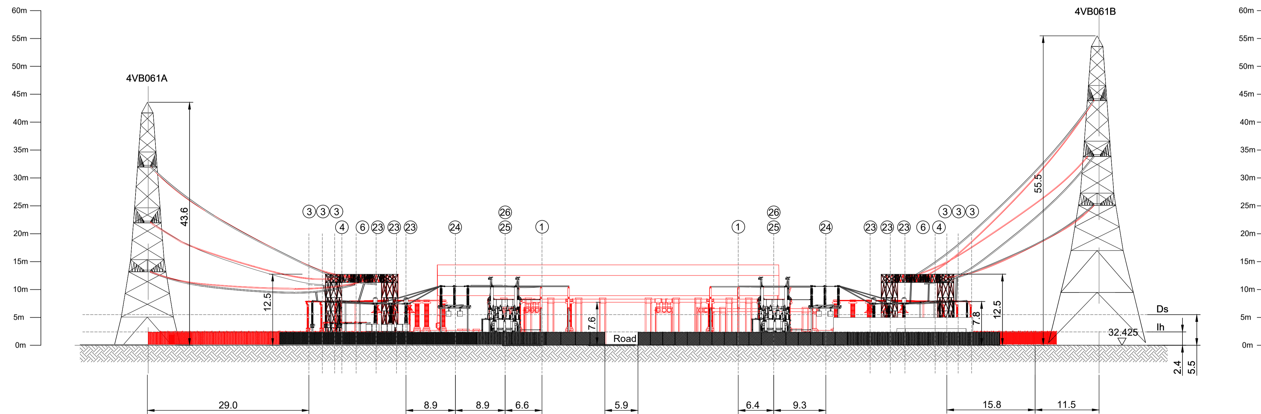
ELEVATION ON E-E
