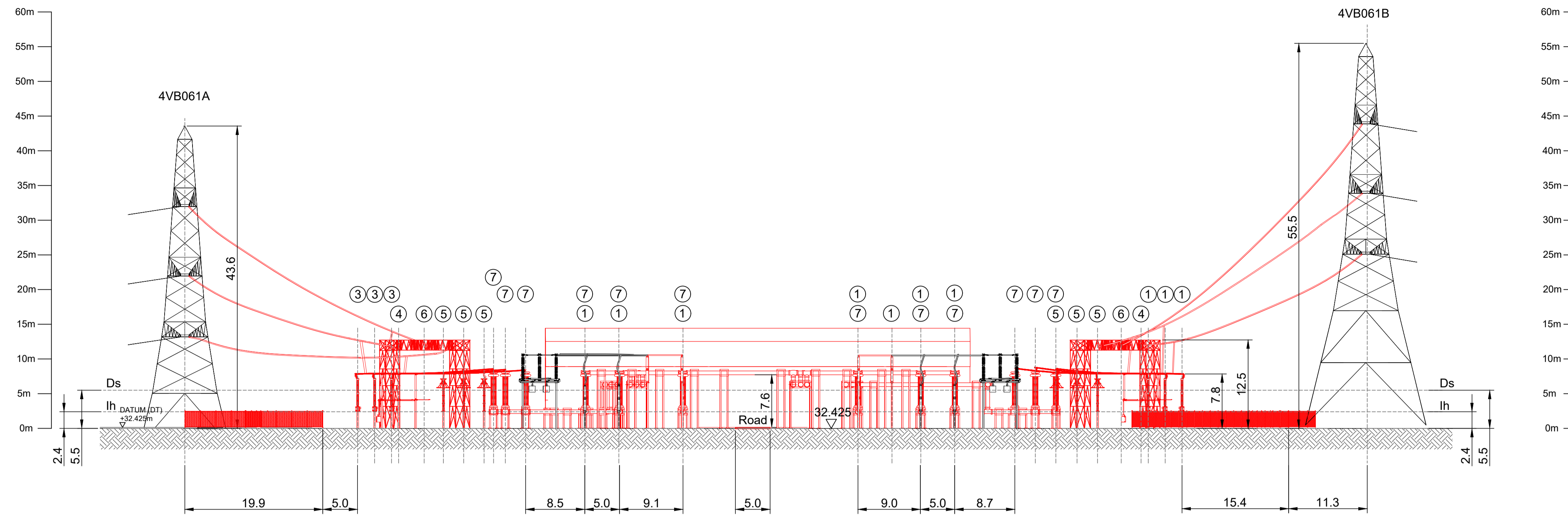
ELEVATION ON D-D
